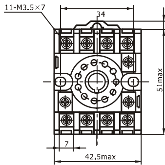
Outline dimensions
