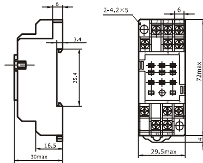
Outline dimensions
