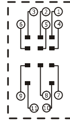
Wiring diagram
