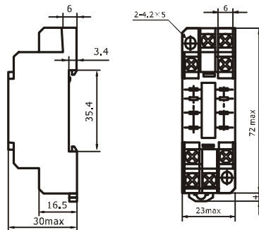
Outline dimensions
