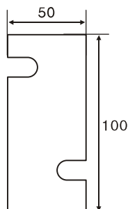
Installation dimensions
