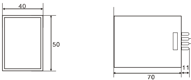
Installation dimensions
