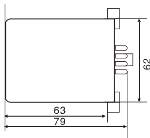
Installation dimensions
